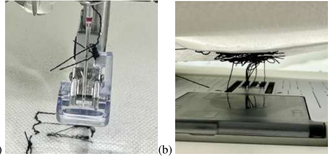
Fig. 3: Errors during the embroidery process: (a) thread breakage and (b) bobbin thread getting stuck under the needle plate.
